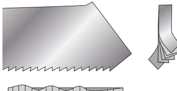
Milled and wavy set teeth.
