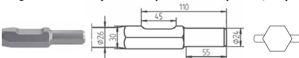
Hexagonal 30 mm + cylindrical tip Ø24x55 mm (ref.393, 394)
