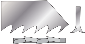
Grinded (or sharpened) and side set teeth.
